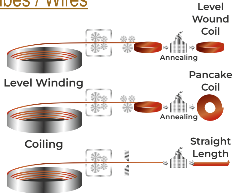
Straightening & Cutting
